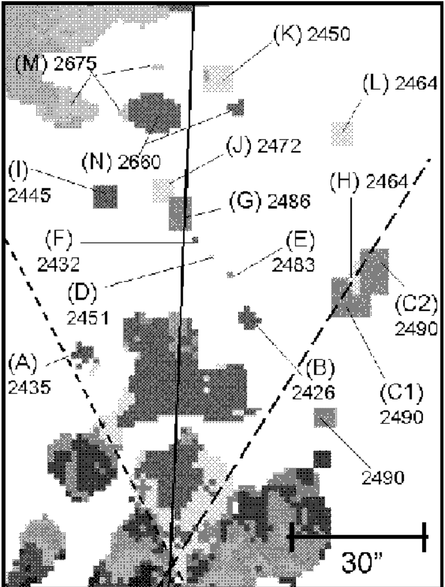
Fig. 4. Velocity field of the bridge-like H_\alpha feature between NGC 5426 and NGC 5427. Letters are related to particular kinematical features in NGC 5426's rotation curve shown in Figure 5.
