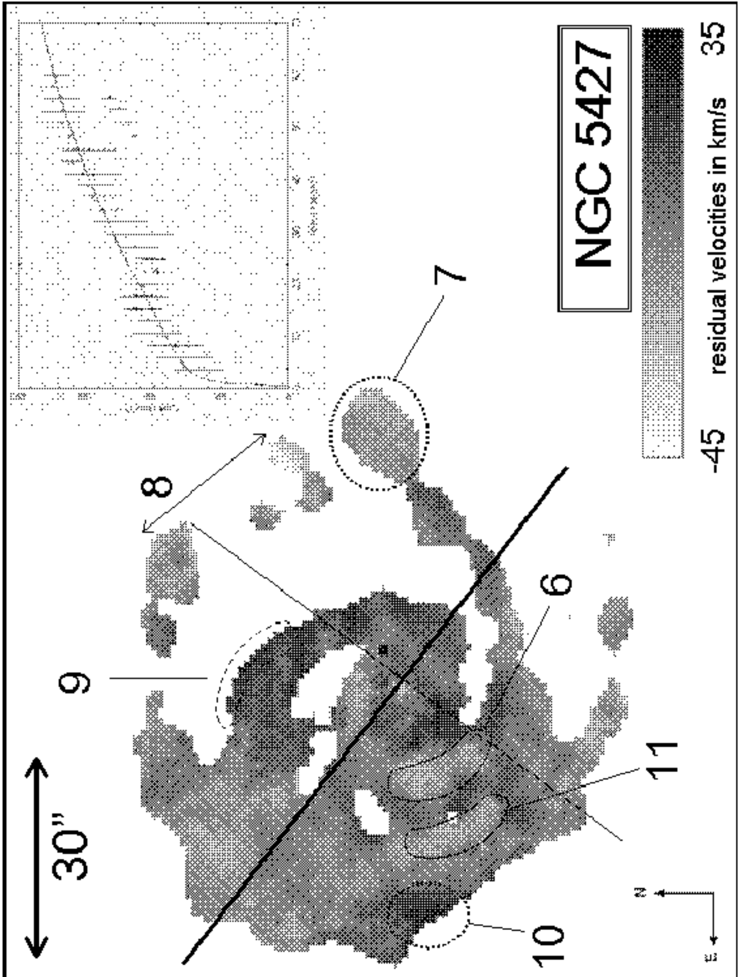
Fig. 11. Residual velocity field of NGC 5427. Upper right panel shows the analytical rotation curve used for the computation of the ideal velocity field. Regions 6 to 11 are discussed in section 5.2.2.
