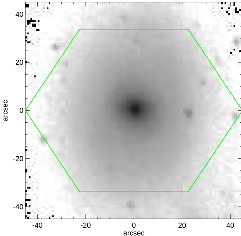
NGC4659
